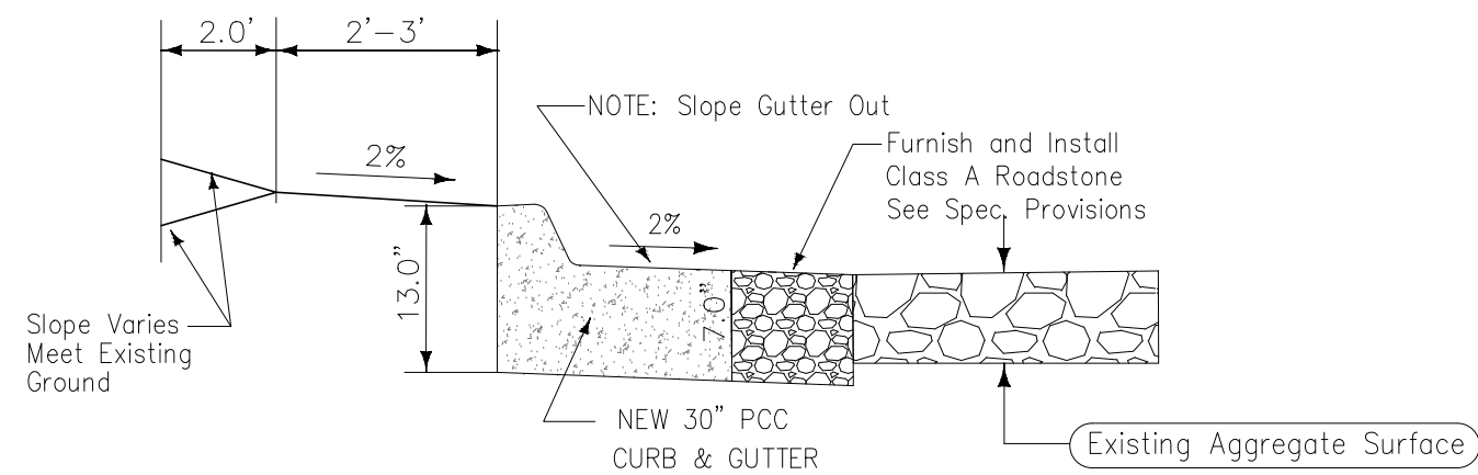
30" PCC CURB & GUTTER DETAIL See Special Provisions
