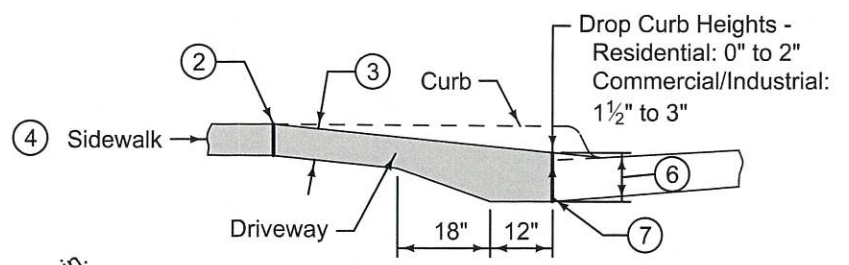
TYPICAL SECTION
