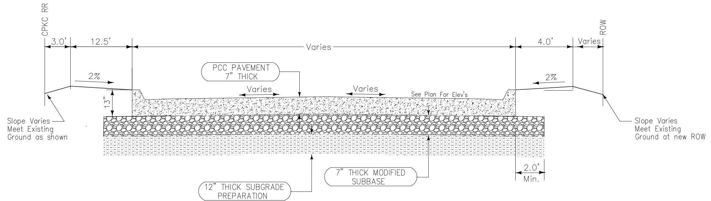
IOWA & LANE STREETS PCC PAVING TYPICAL SECTION
