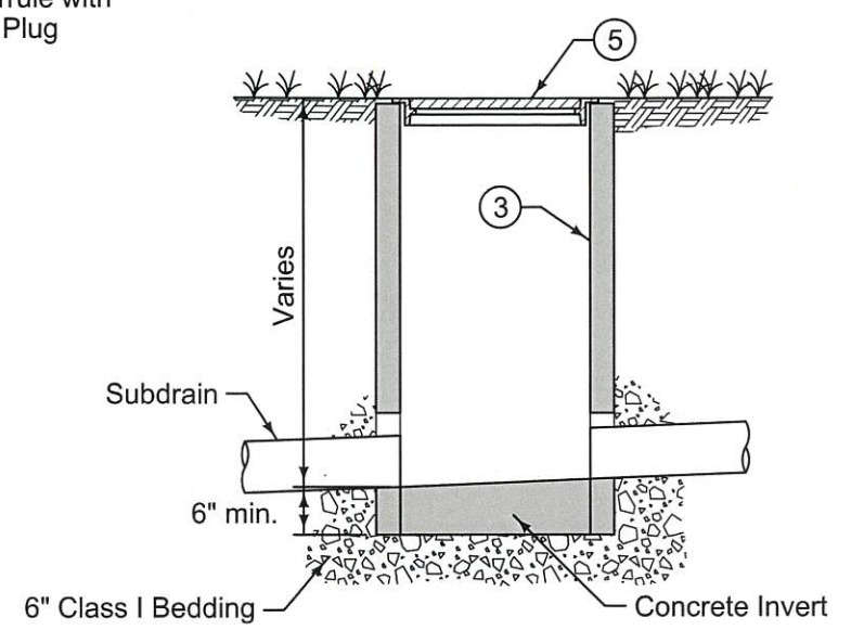
TYPE B CLEANOUT
