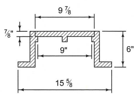
DETAIL A (1) (4) (Dimensions are nominal)
