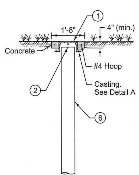
TYPE A-1 CLEANOUT
