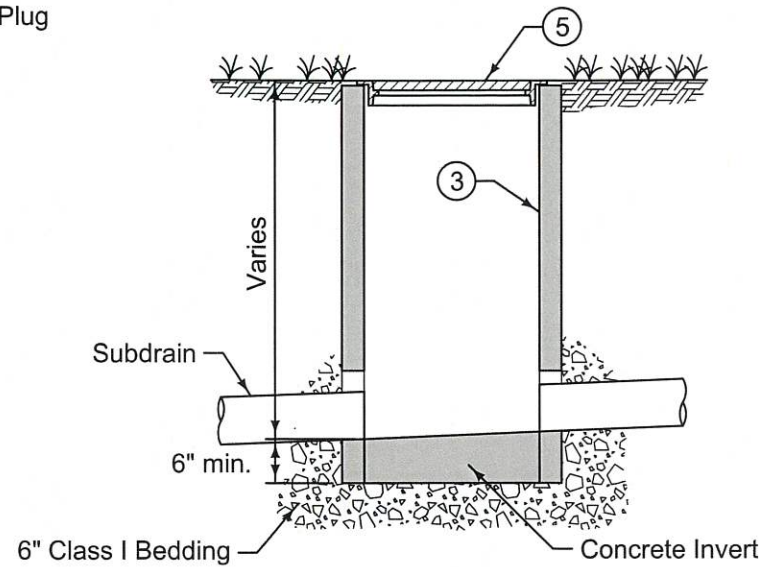
TYPE B CLEANOUT
