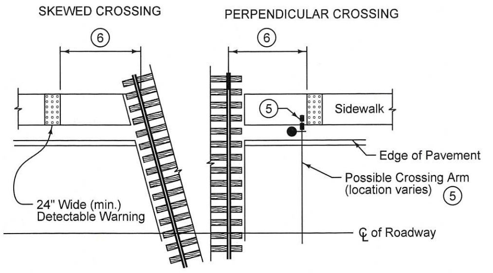
DETECTABLE WARNING LOCATION AT RAILROAD CROSSING
