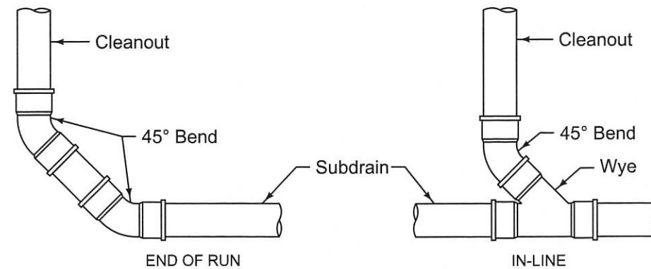
TYPE A CLEANOUT CONNECTIONS
