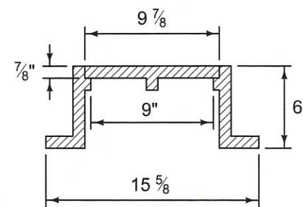
DETAIL A ① ④ (Dimensions are nominal)
