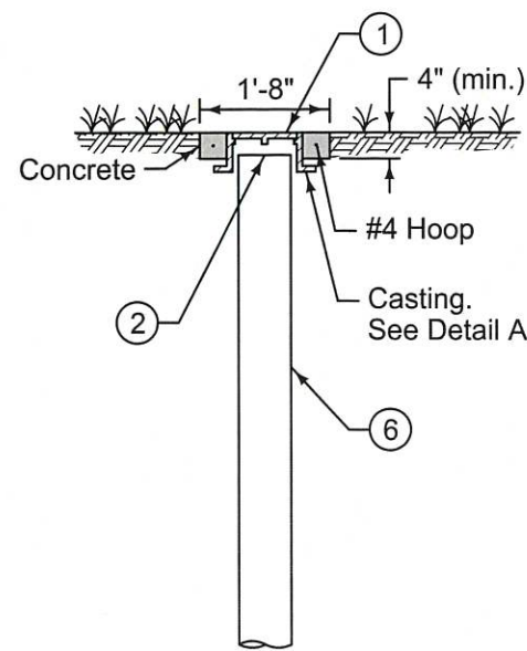
TYPE A-1 CLEANOUT
