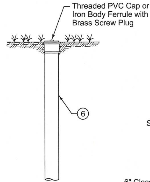
TYPE A-2 CLEANOUT
